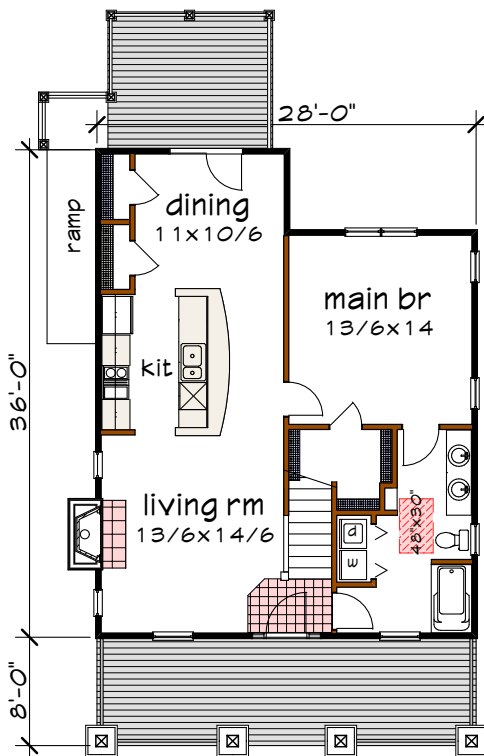
Floor 1 plan
