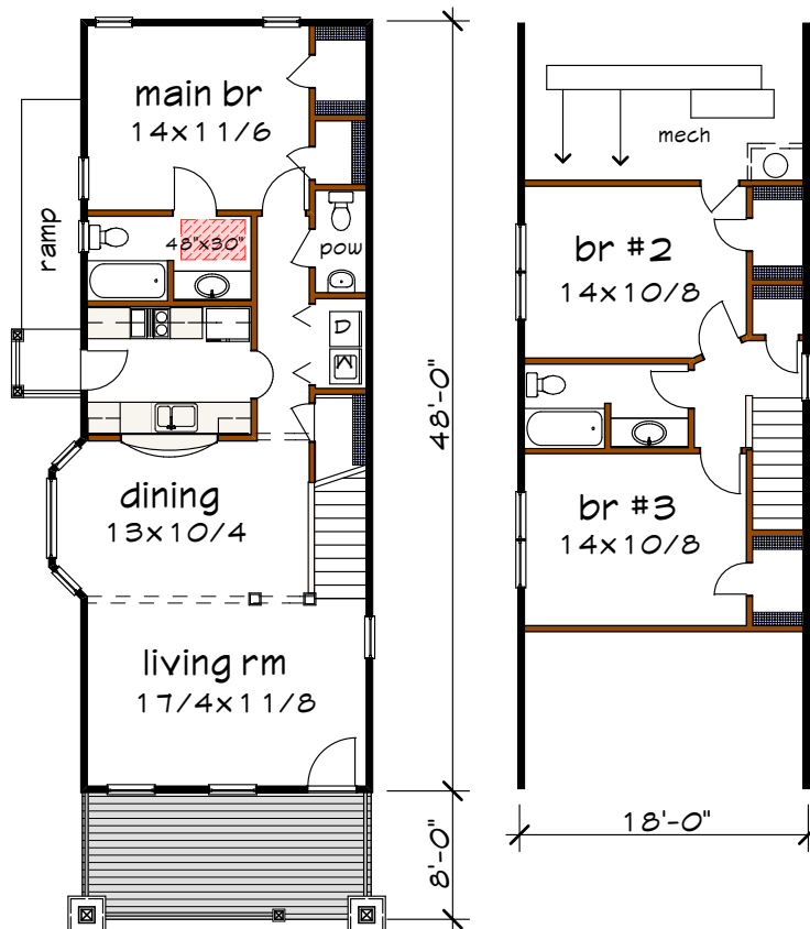
Floor 1 plan
