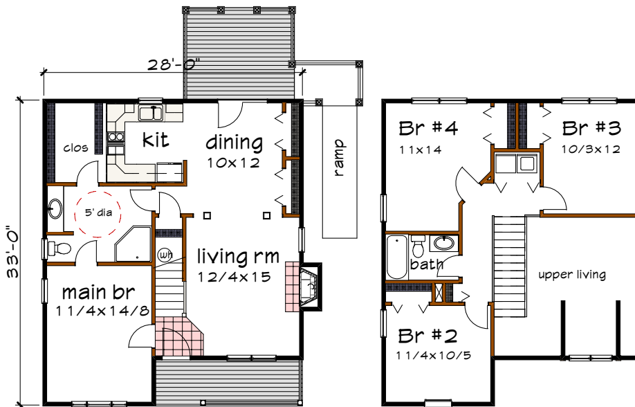
Floor 1 plan
