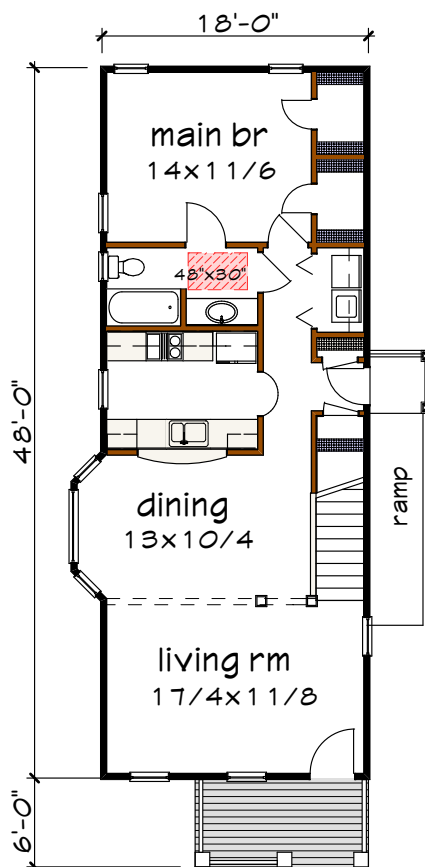
Floor 1 plan
