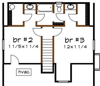
Floor 2 plan
