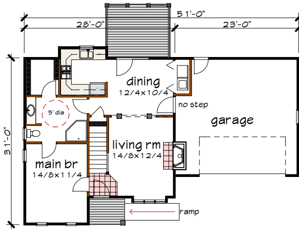
Floor 1 plan
