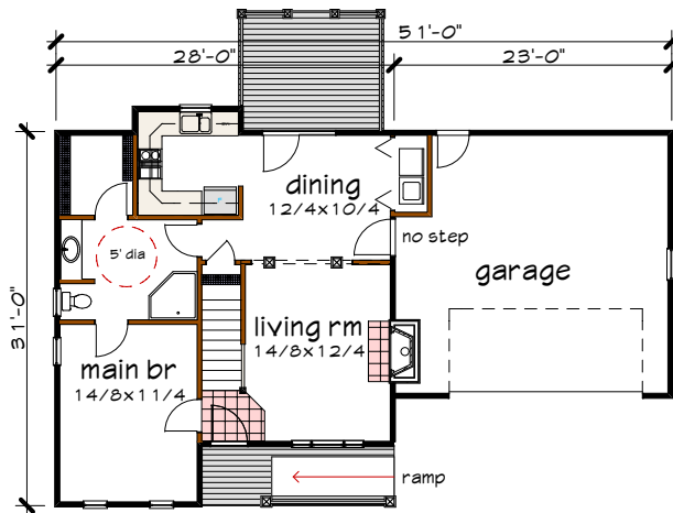
Floor 1 plan
