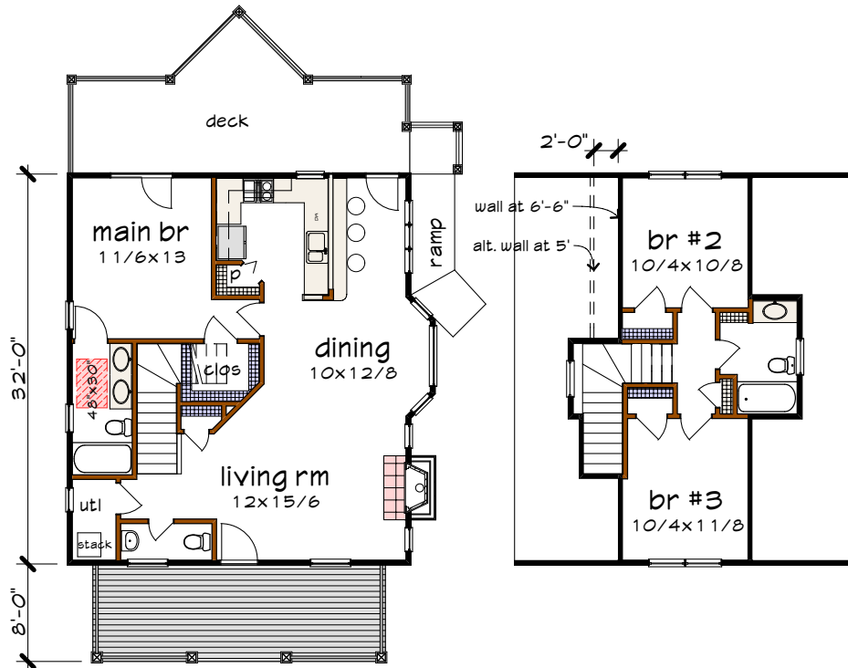
Floor 1 plan
