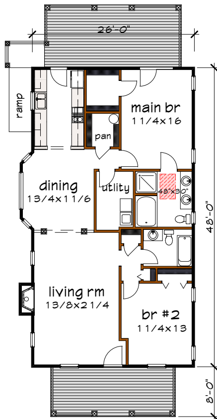
Floor Plan
