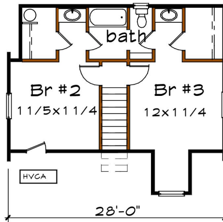
Floor 2 plan
