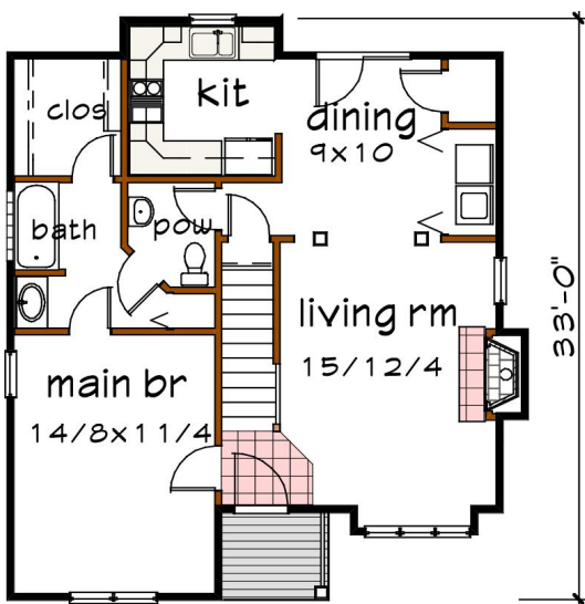
Floor 1 plan
