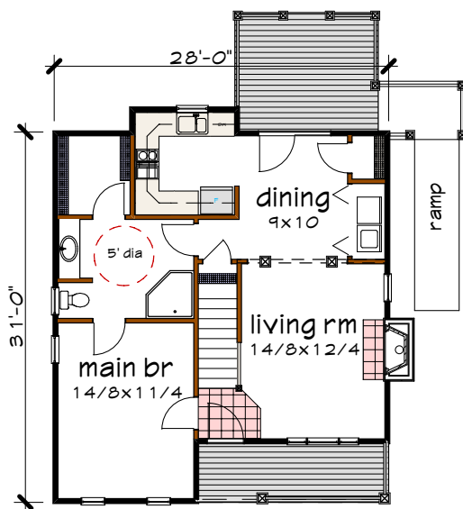
Floor 1 plan
