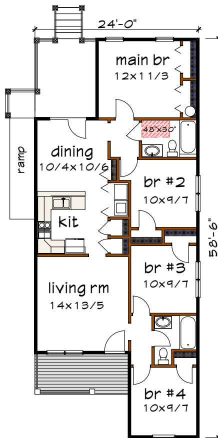
Floor 1 plan
