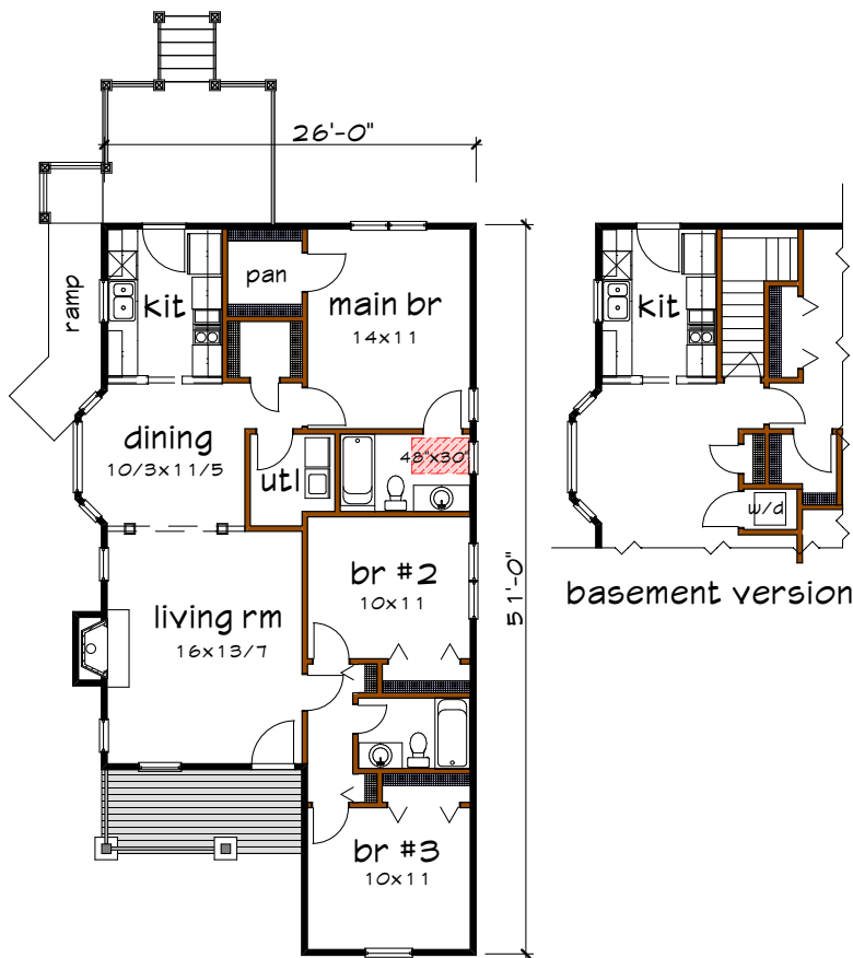
Floor 1 plan
