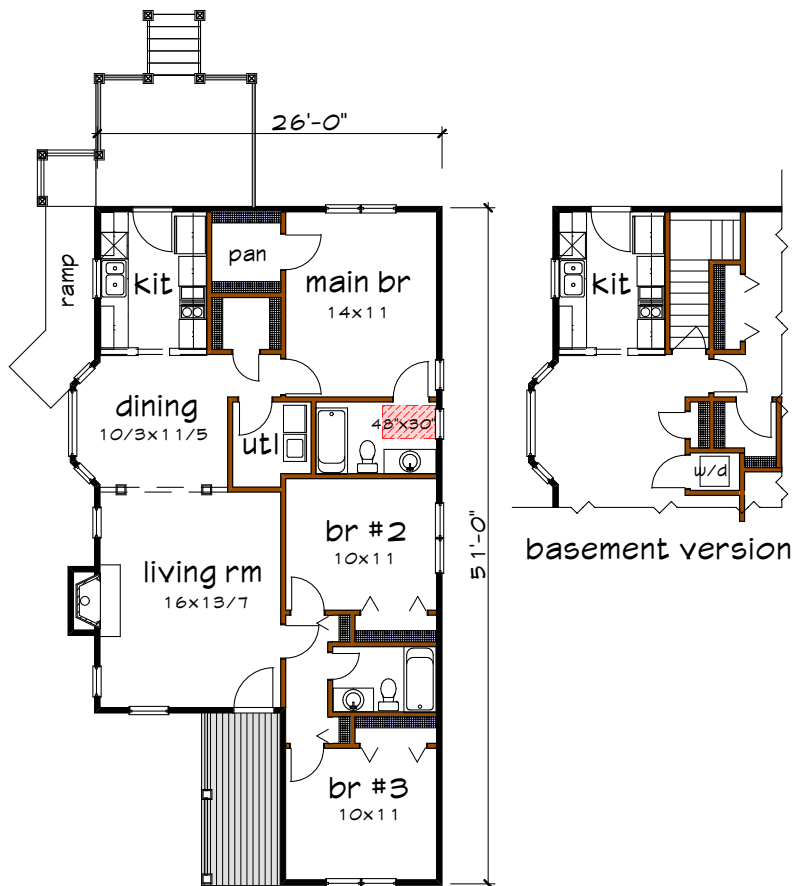
Floor 1 plan
