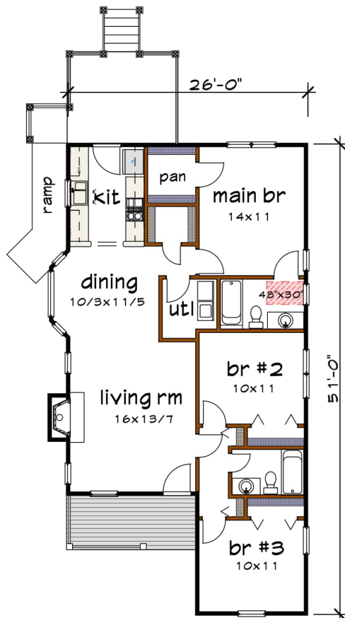
Floor 1 plan
