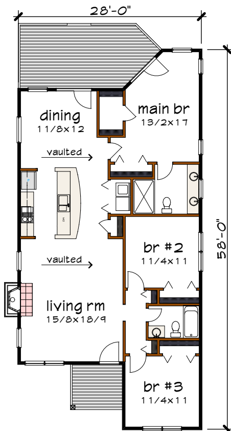
Floor 1 plan
