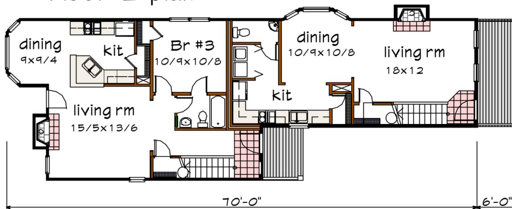
Floor 1 plan
