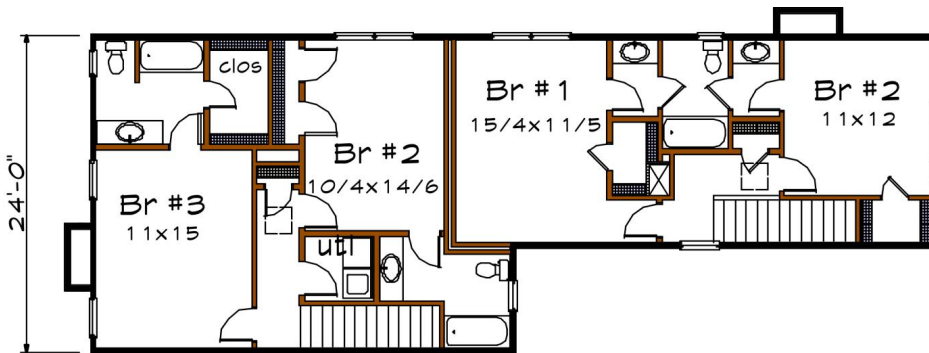
Floor 2 plan
