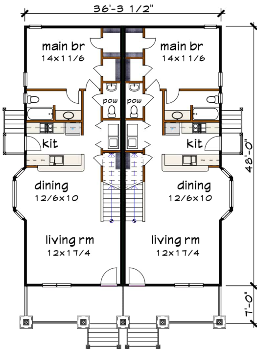
Floor 1 plan
