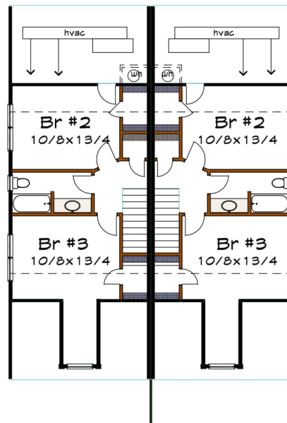
Floor 2 plan
