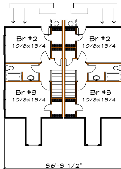
Floor 2 plan
