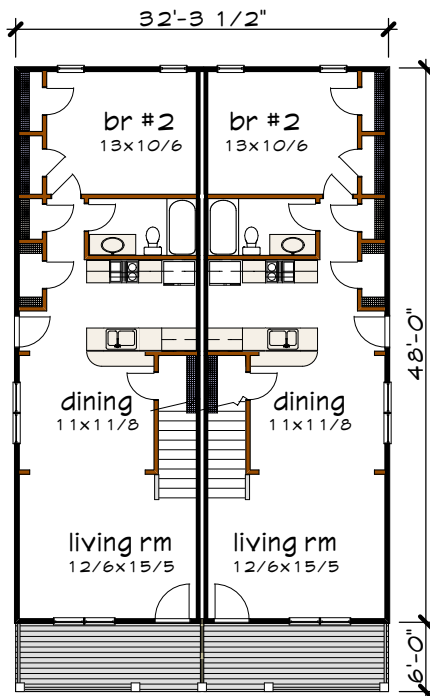
Floor 1 plan
