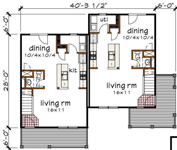
Floor 1 plan
