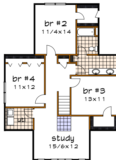
Floor 2 plan
