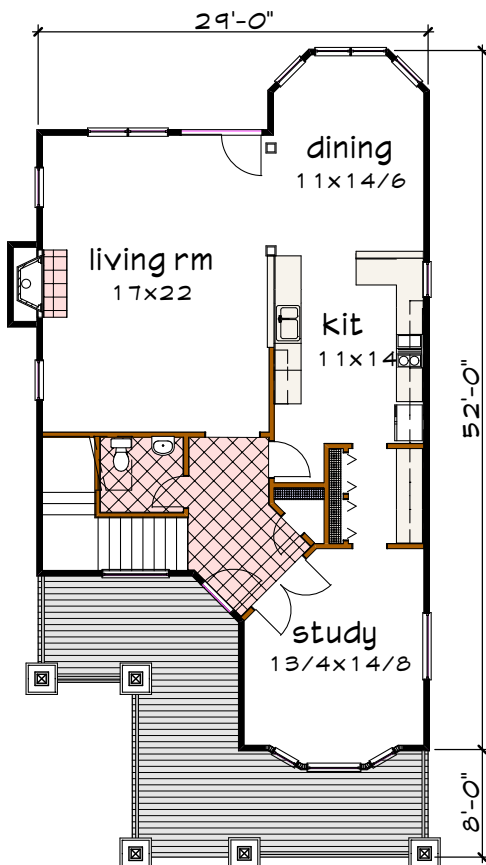
Floor 1 plan
