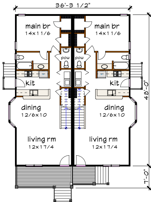
Floor 1 plan
