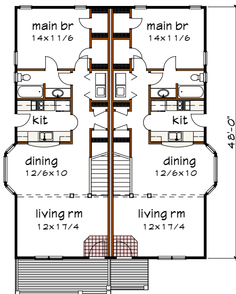
Floor 1 plan
