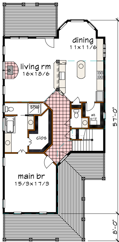
Floor 1 plan
