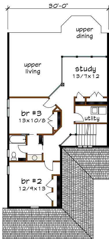
Floor 2 plan
