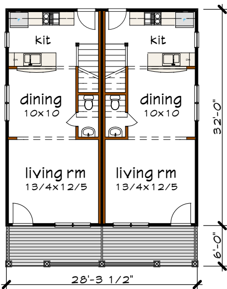
Floor 1 plan
