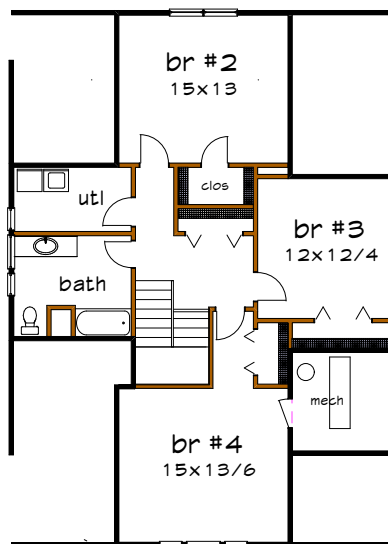
Floor 2 plan
