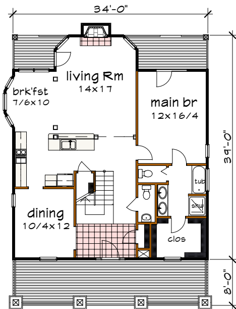
Floor 1 plan
