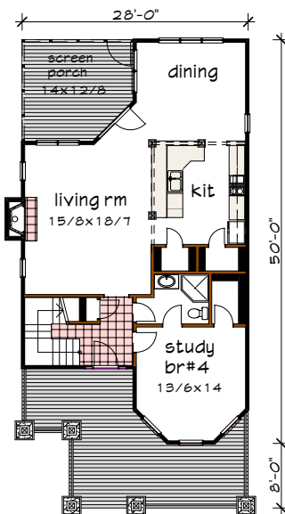
Floor 1 plan
