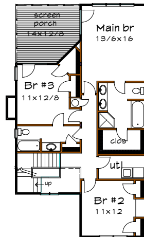
Floor 2 plan
