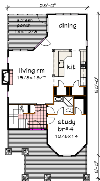
Floor 1 plan
