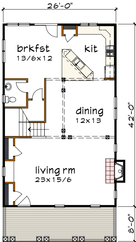
Floor 1 plan
