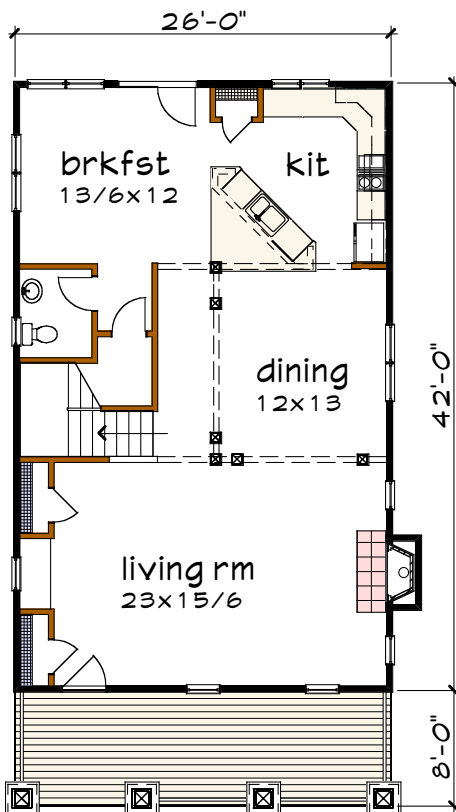
Floor 1 plan
