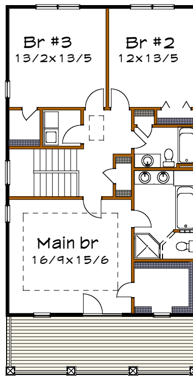
Floor 2 plan
