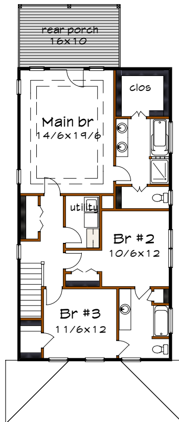
Floor 2 plan
