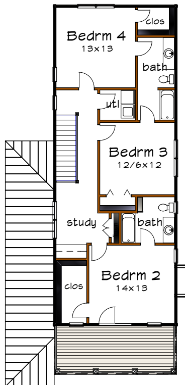
Floor 2 plan
