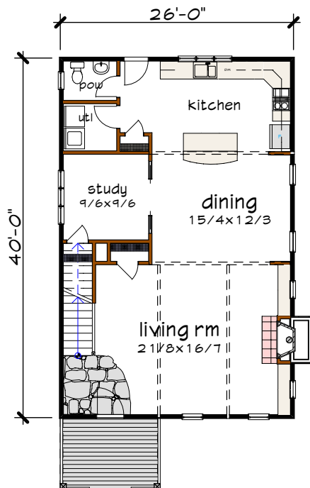
Floor 1 plan
