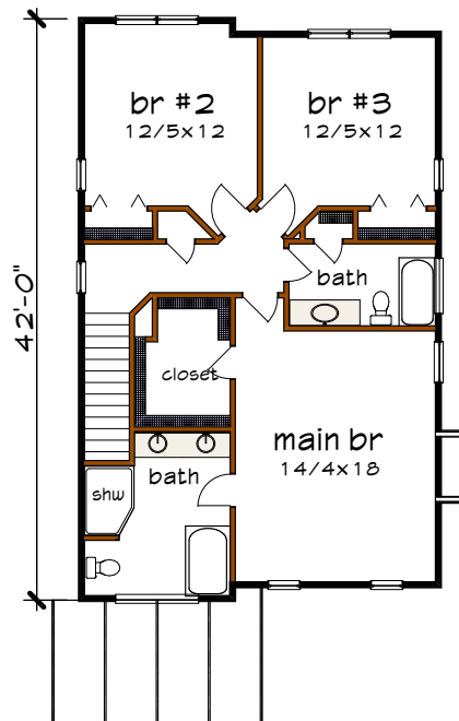
Floor 2 plan
