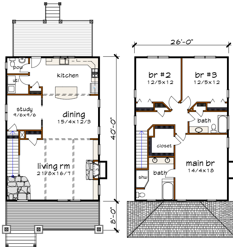
Floor 1 plan
