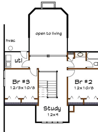
Floor 2 plan
