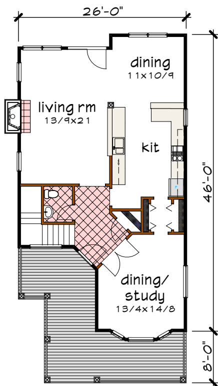
Floor 1 plan
