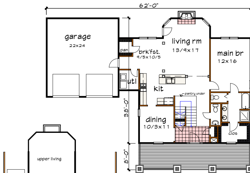
Floor 1 plan
