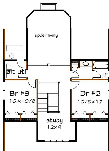
Floor 2 plan
