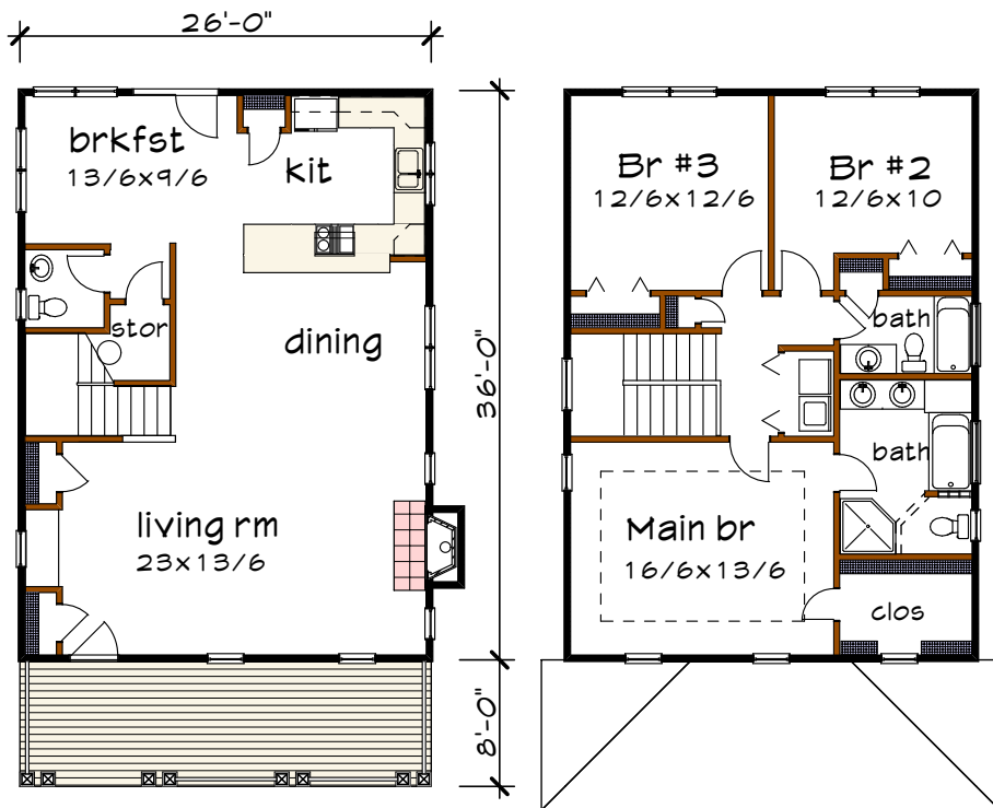
Floor 1 plan
