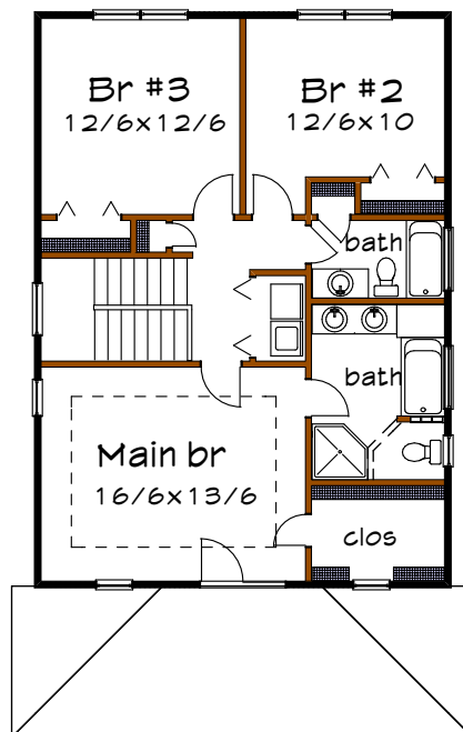
Floor 2 plan
