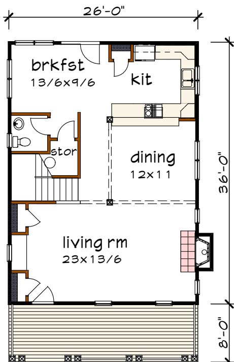
Floor 1 plan
