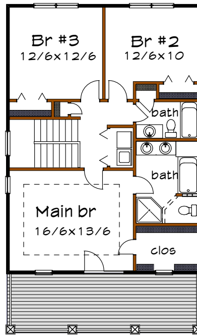
Floor 2 plan
