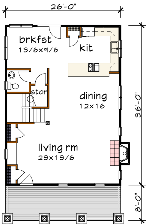
Floor 1 plan
