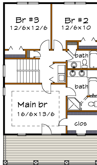
Floor 2 plan
