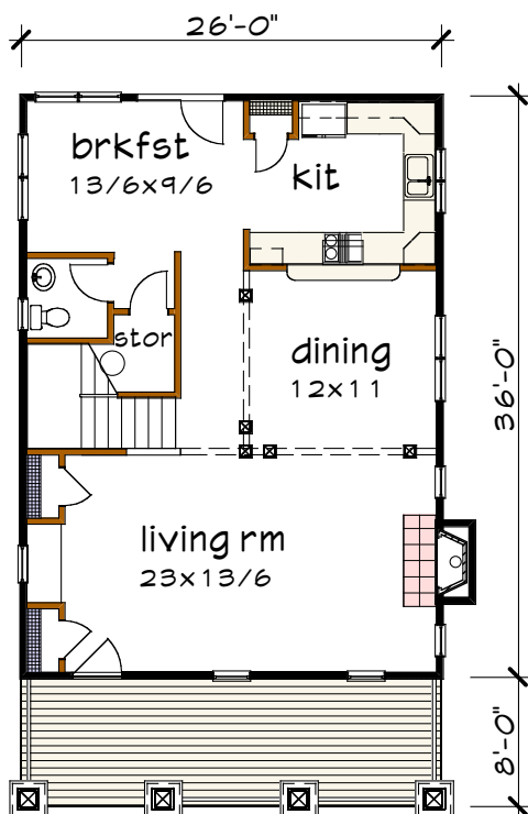
Floor 1 plan
