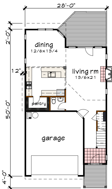
Floor 1 plan
