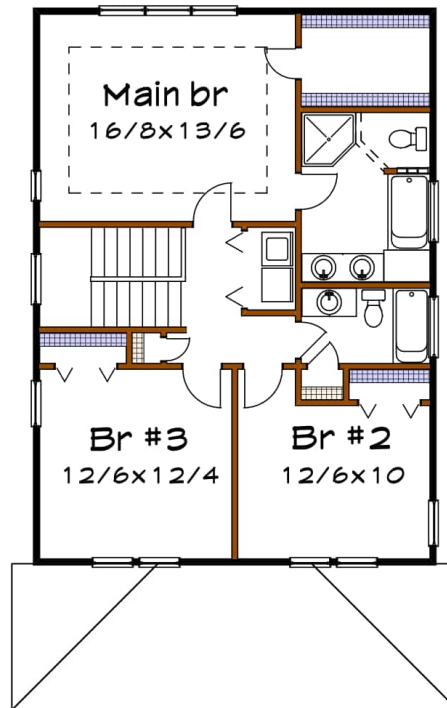
Floor 2 plan
