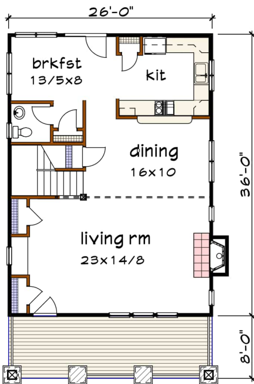
Floor 1 plan
