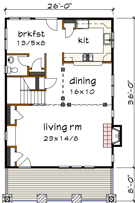
Floor 1 plan
