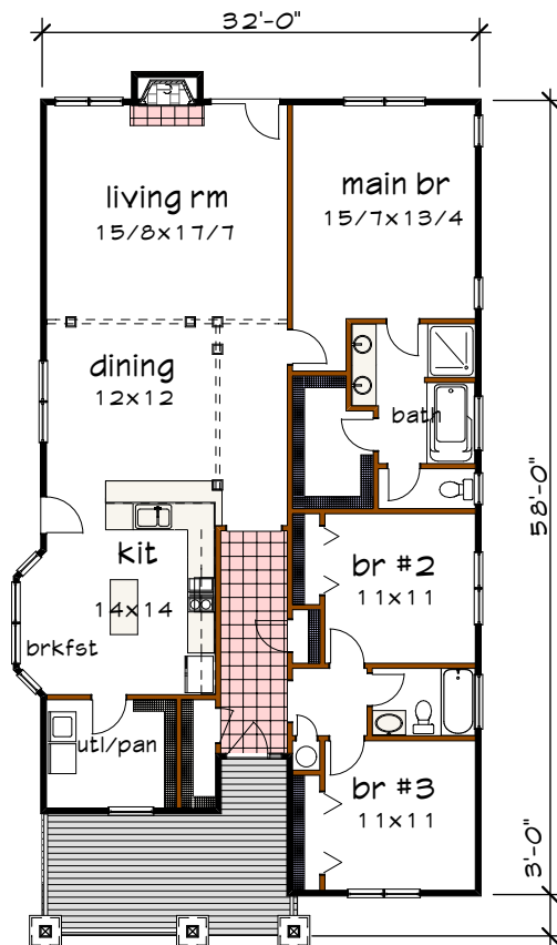
Floor plan
