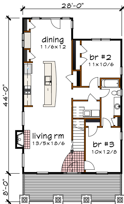
Floor 1 plan
