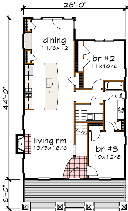
Floor 1 plan
